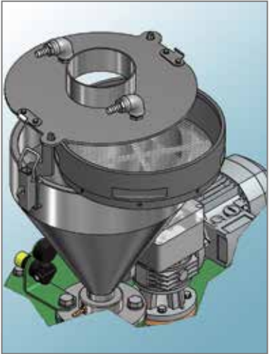
Vezin Sampler with Tramp Material Screen
